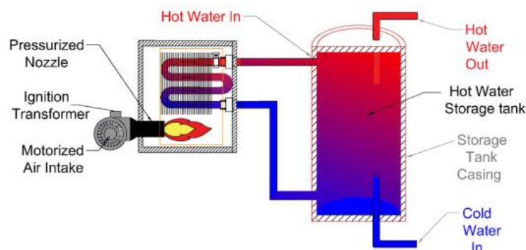
Figure 2-4: Oil-fired water heater (Hohne, Kusakana and Numbi, 2019)
