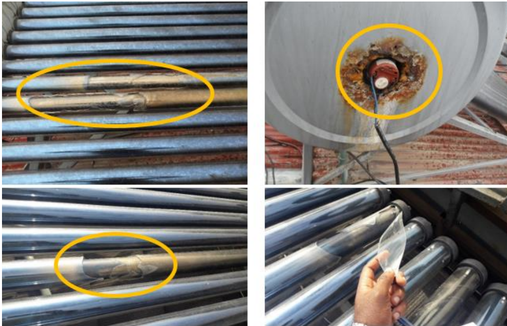
Figure 4-22: Evacuated tube collector type SWH under poor working condition
