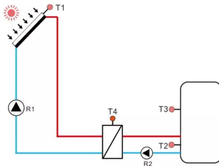
Figure 3-7: Design approach four: 6,000L-12,000L SWH system
