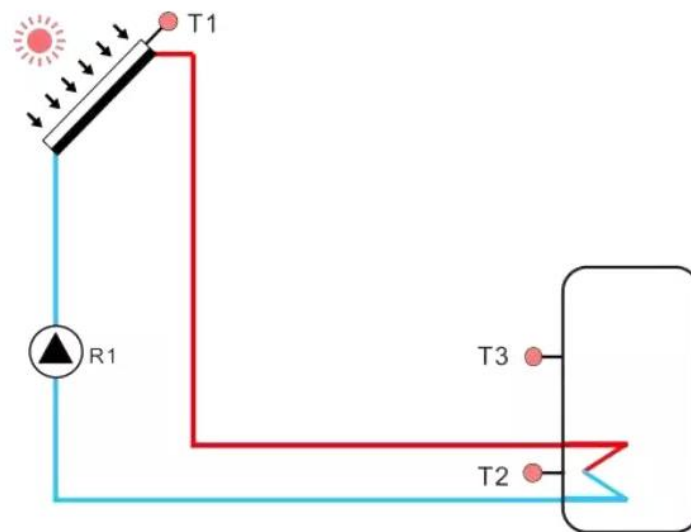
Figure 3-6: Design approach three: 3,000L-5,000L SWH system
